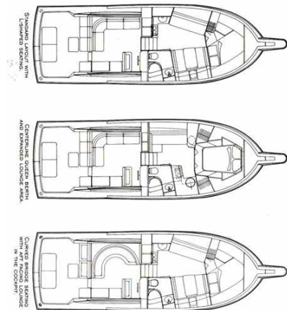
Hatteras 39 Express lay out
