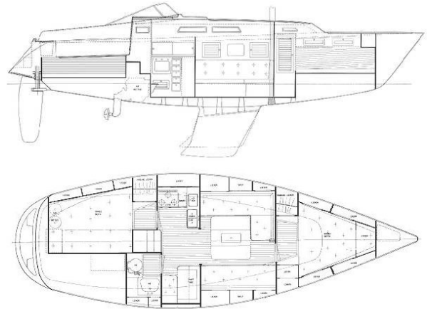
hallberg-rassy_34_drawing
